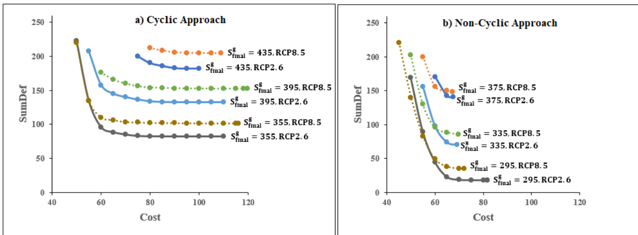
Fig. 5- Performance (a) CSS and (b) NCSS under RCP2.6 and RCP8.5 (Ensemble model)
