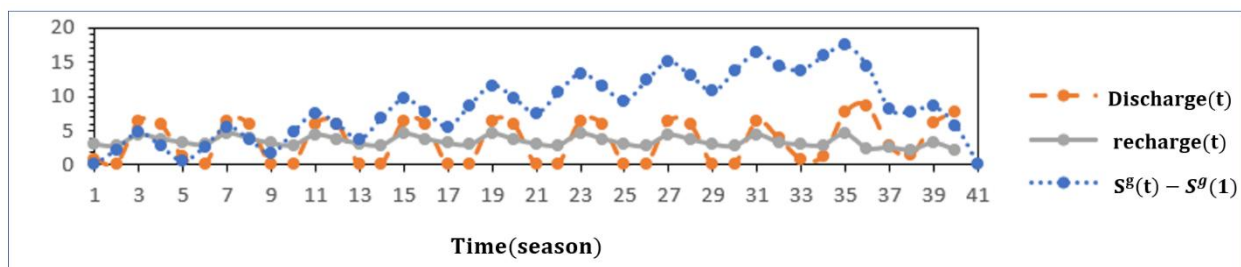
Fig. 7- Values of recharge, discharge and the aquifer storage volume in cyclic operation (MCM)
