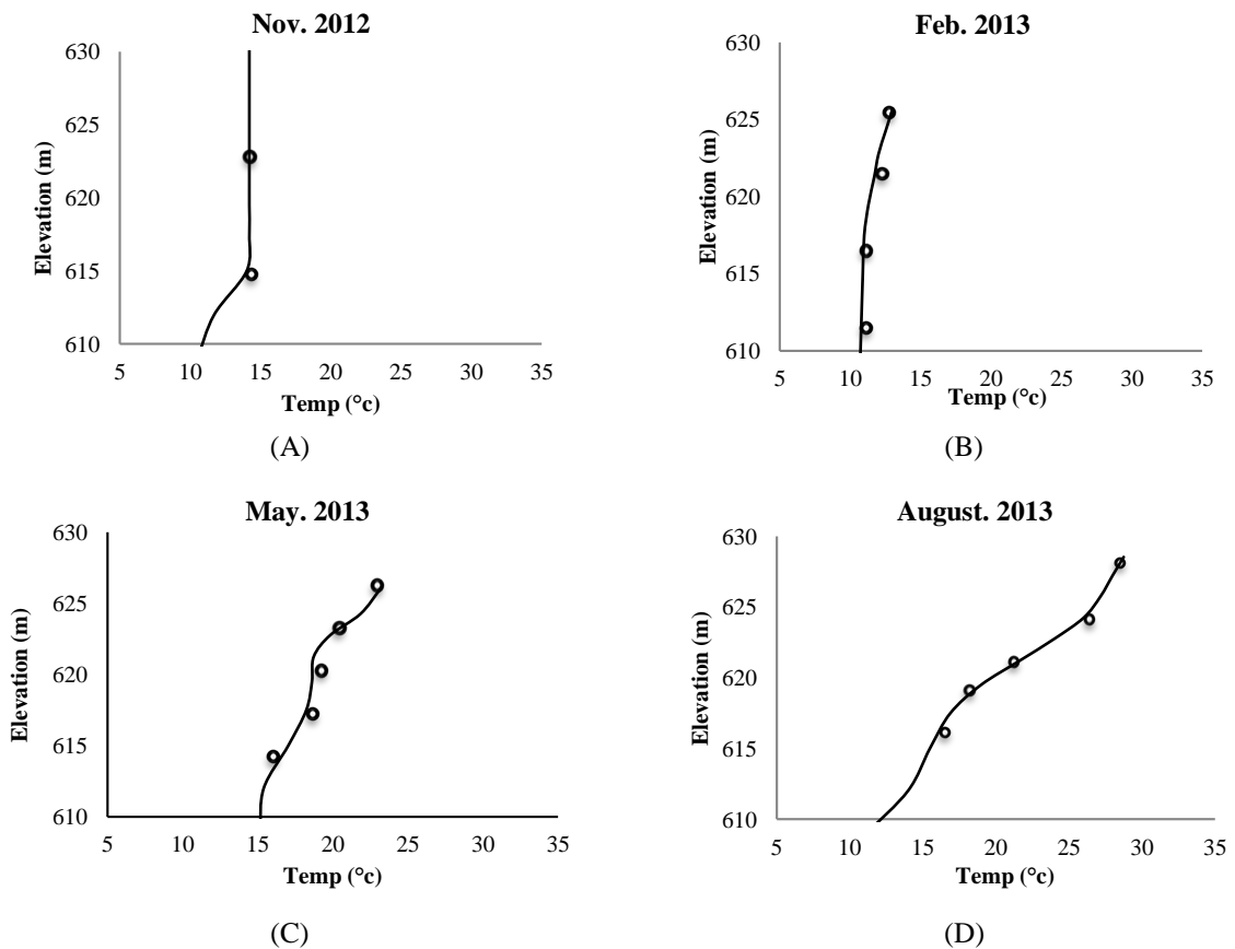
Fig. 7 - Calibration results of temperature in S2 station
