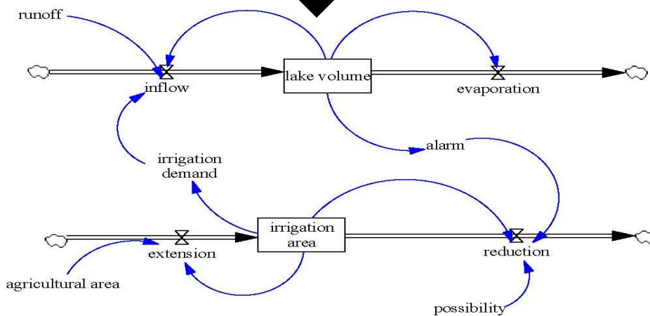
Fig. 7- (A) The stock and flow diagram designed in VENISM software and (B) predator- prey model for Urmia Lake
