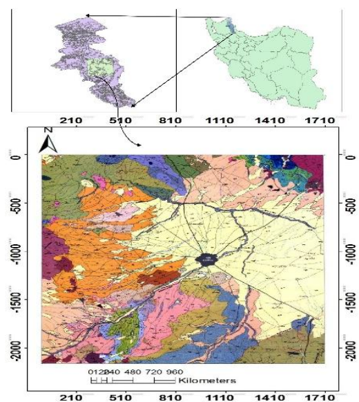
Fig. 1- Location of studied basin and geological view of Ardebil
