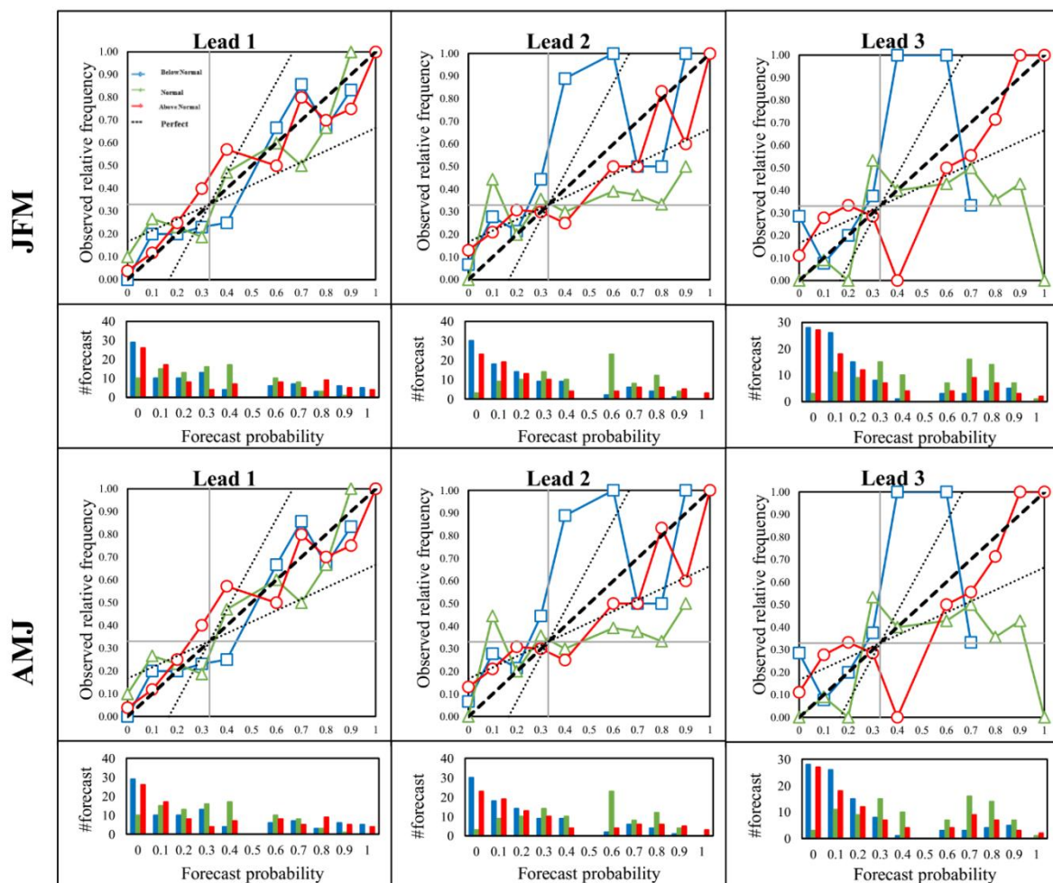
Fig. 4- Two season (JFM, AMJ) Reliability diagrams and sharpness for the seven models of NMME precipitation forecast
