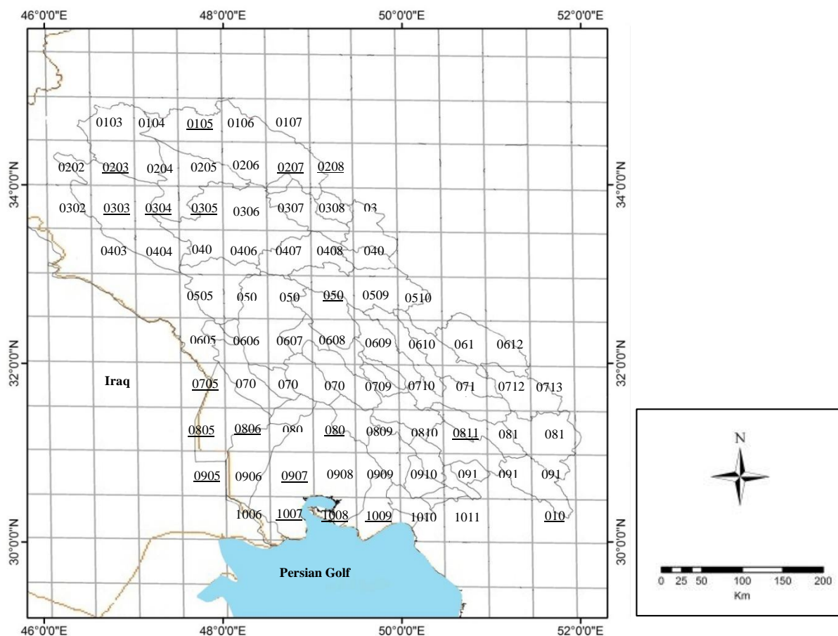
Fig. 2-Geographical location of grid cells used for postprocessing of CFSv.2 model
