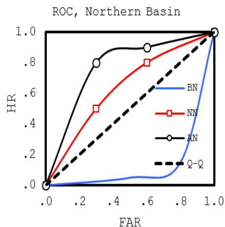
Fig. 6- ROC curve for Bellow Normal (BN), Normal (NN) and Above Normal (AN) categories in north of basin
