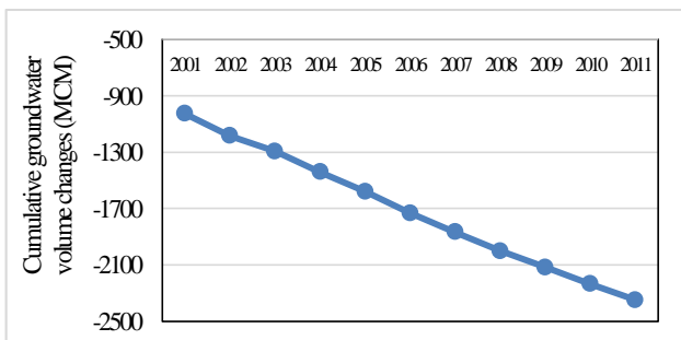
Fig. 2- Cumulative changes in groundwater (Iran Water Resources Management Company, 2012)
