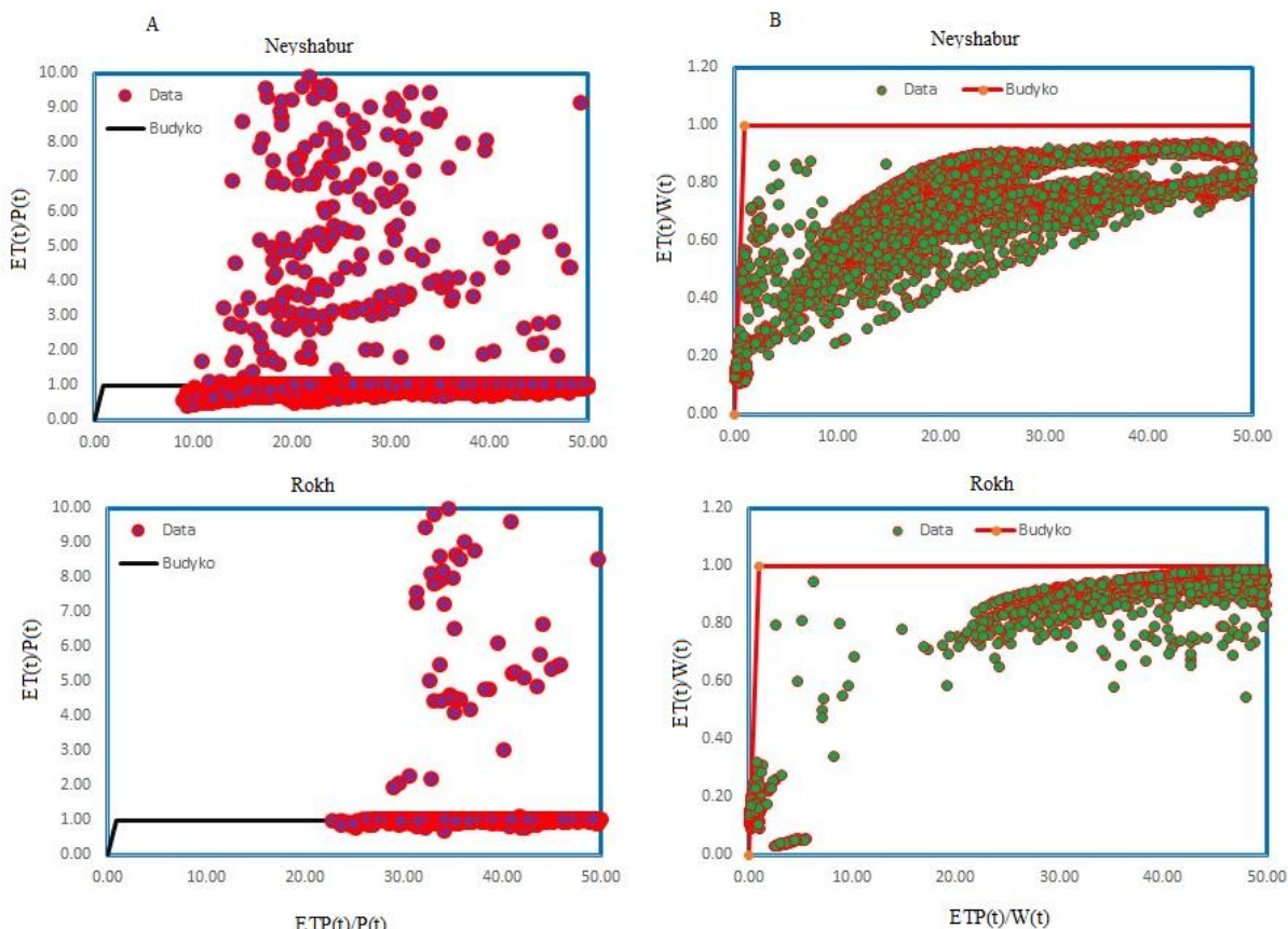
Fig. 6- Model performance based on the Budyko Curve in study areas *
