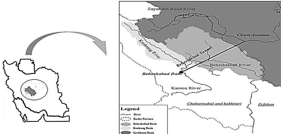
Fig. 4- The map of the study area
