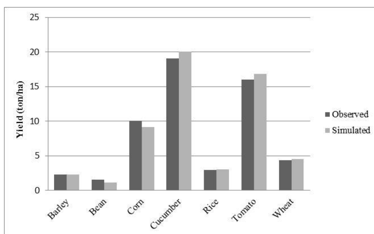
Fig. 4- Comparison between simulated and observed yield of the crops
