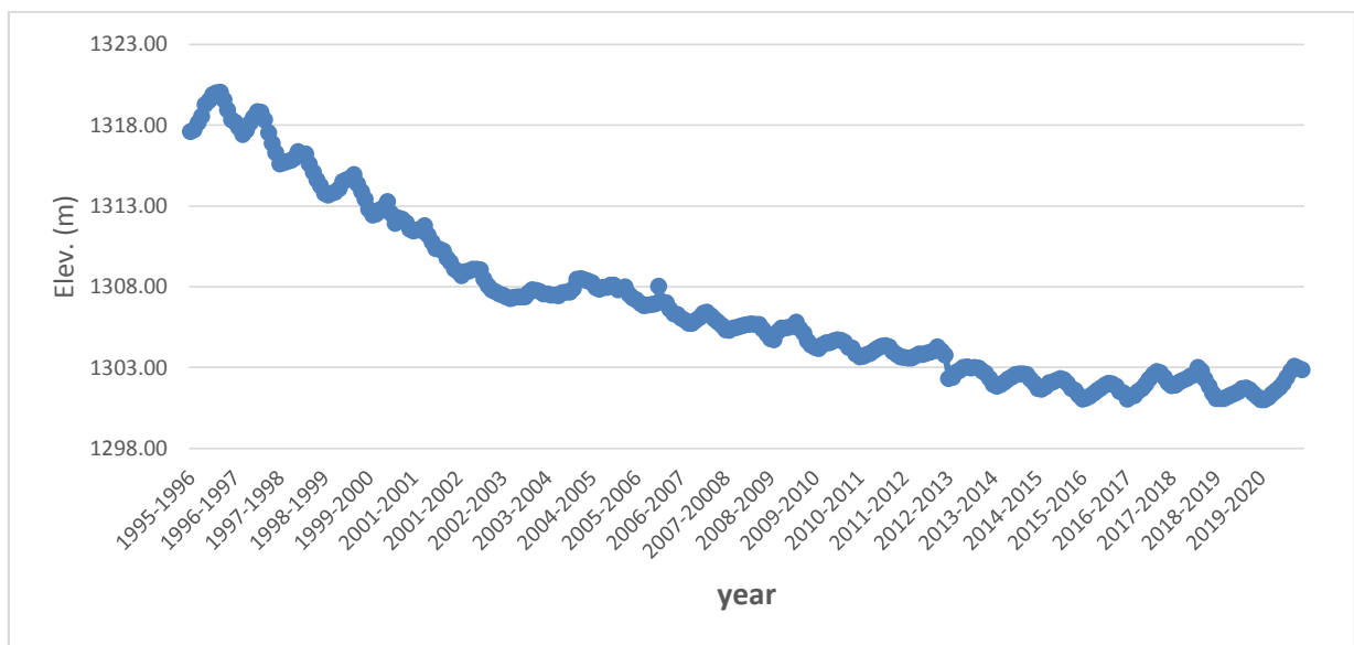
Fig. 4 – Hydrograph of alluvial aquifer Tasuj (Code 3024)
